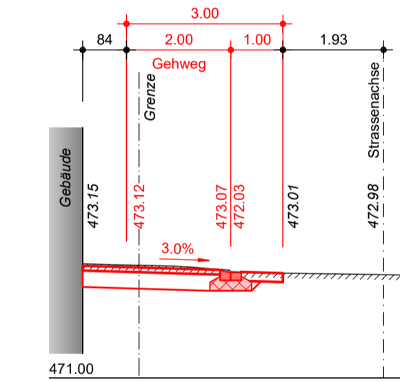
Querprofil 16, 1:100 (150.00 m)
